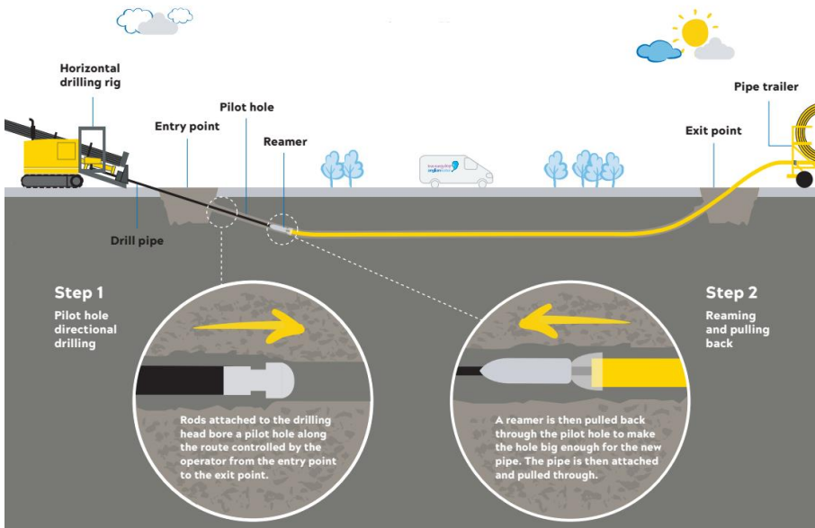
Figure 3.4: Example of a trenchless technique
